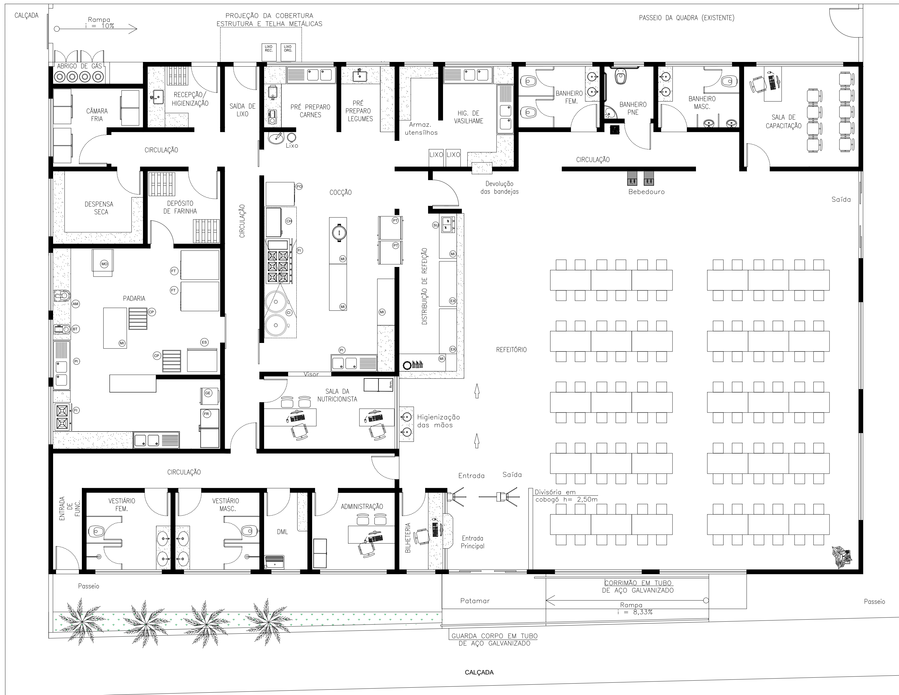
LAYOUT ESC 1/75
